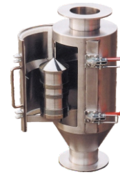
Bullet Magnet
